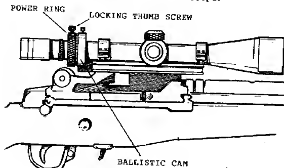
Figure 2-14. ART I scope.
